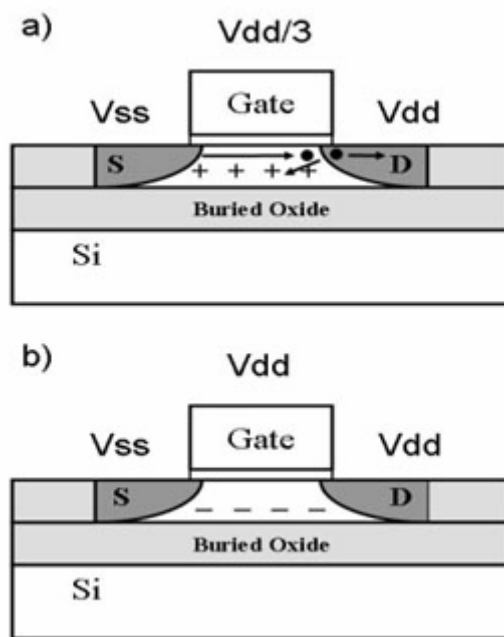
شکل 9: Floating Body Effect و ZRAM : "1" , b : "0" : "1"
